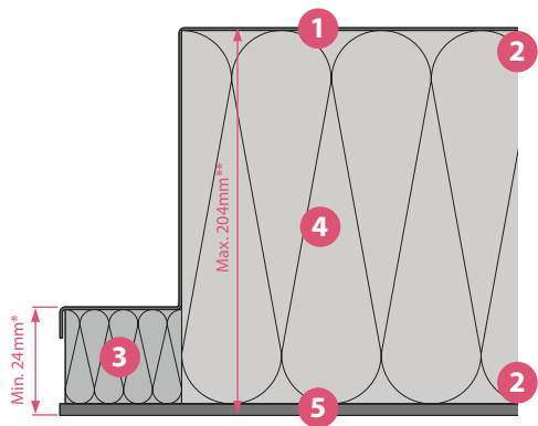
Stepped Rear Spandrel Panel
