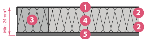
Flat Spandrel Panel
