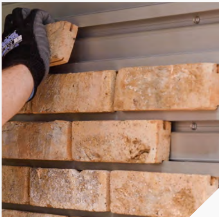
Stage 5 Insert the bricks top edge first, rotate in the bottom edge and engage into the carrier tongue, then pull down the brick to fully engage.
